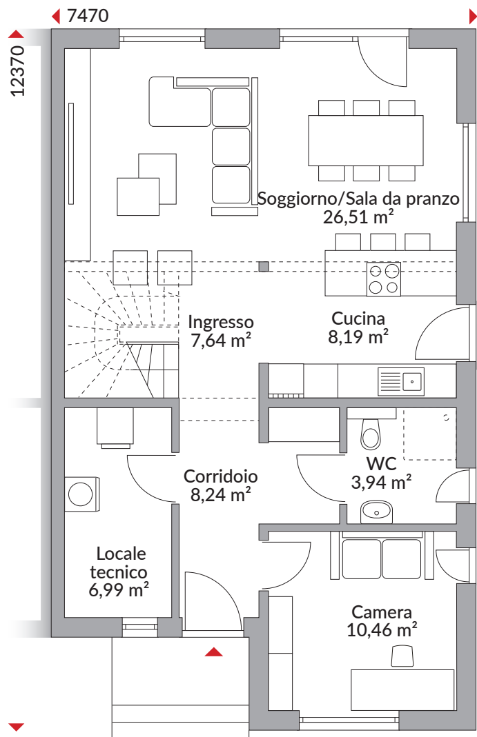
Piano terra 71,97 m 2
