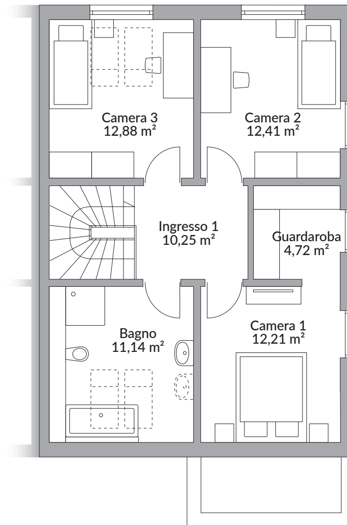
Piano mansarda 63,61 m 2
