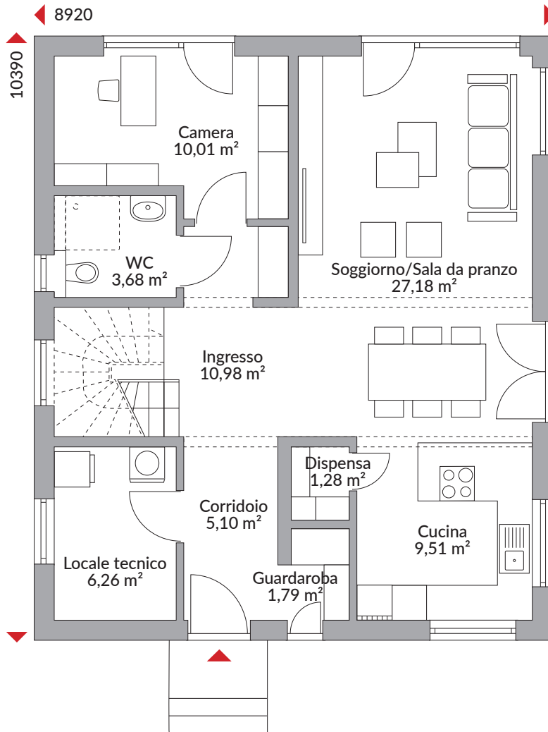
Piano terra 75,79 m 2
